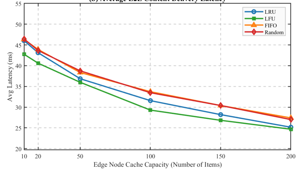
(b) Average E2E Content Delivery Latency
